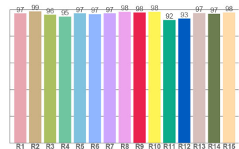
CRI: 96.9 (R1-R8)
